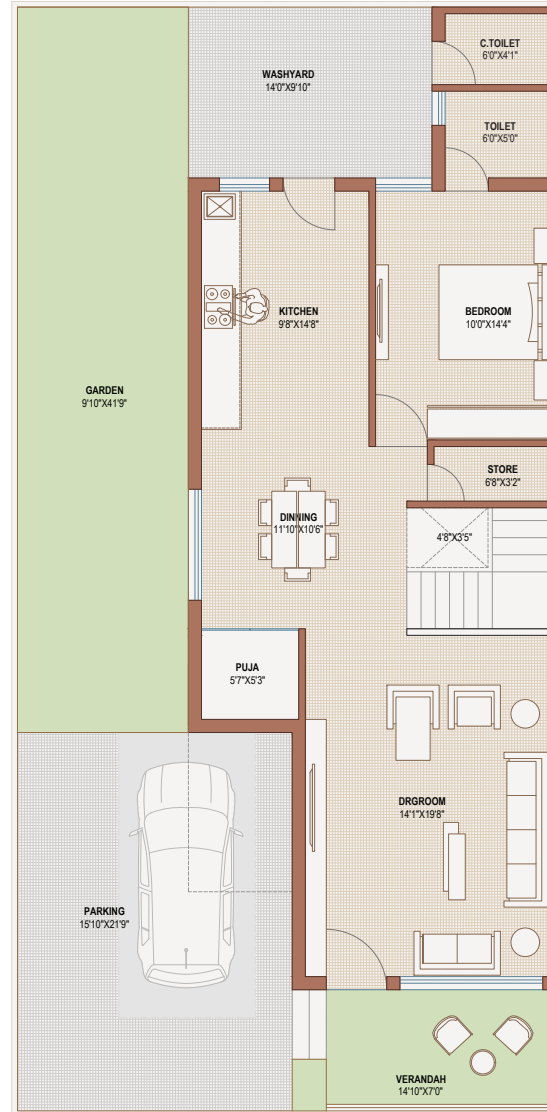
GROUND FLOOR
